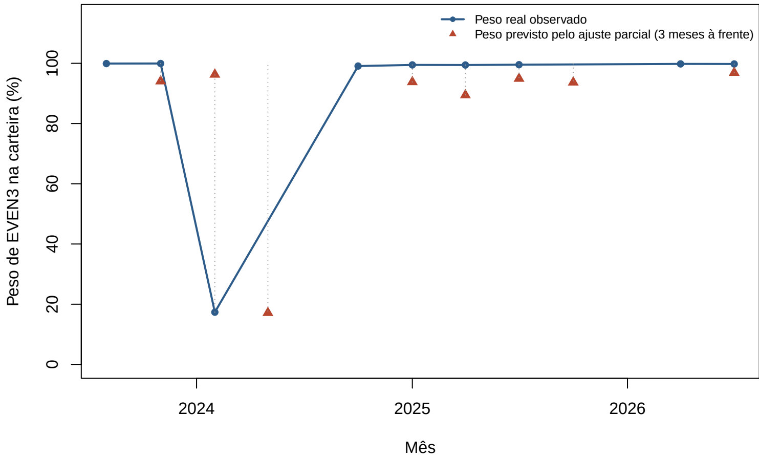
Fundo 46.246.621/0001-50 () --- peso real vs. previsto (h=3)
